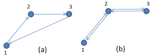
Figure 3: Network example 3
